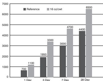
Eucan 1037 Compressive Strenght Data (psi)
