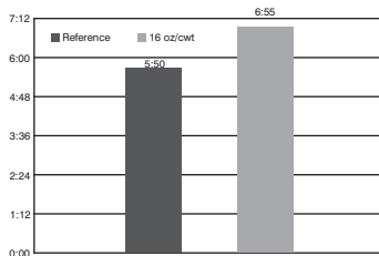
Eucan 1037 Set Time Results (hr:min)
